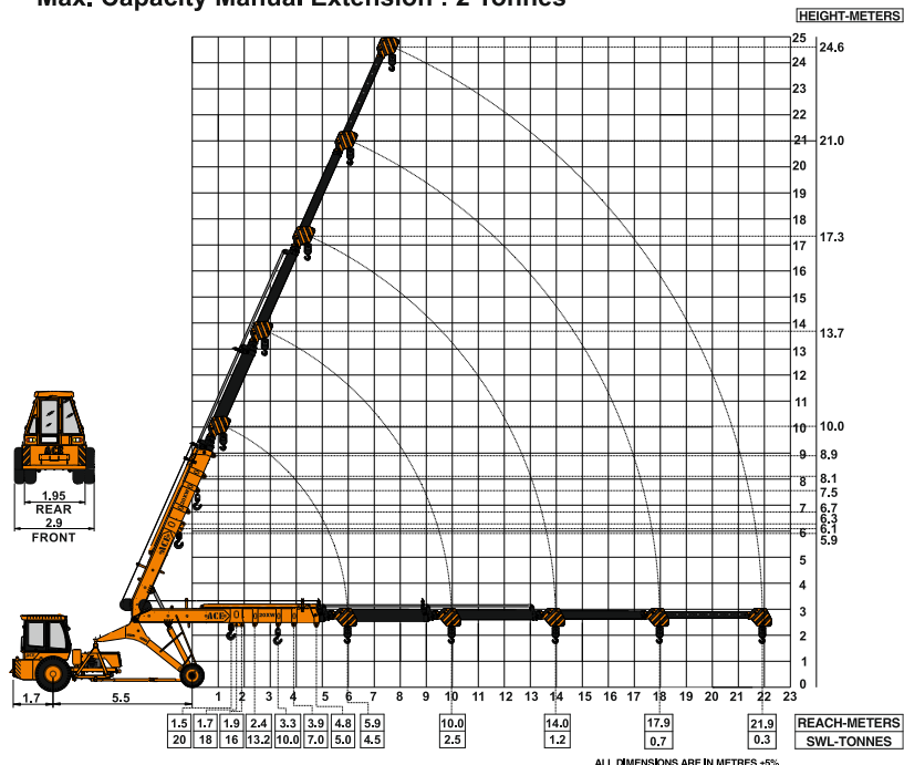
ACE 20XW 5-Part Boom (24.6 mtrs. height) Max. Capacity Manual Extension : 2 Tonnes
