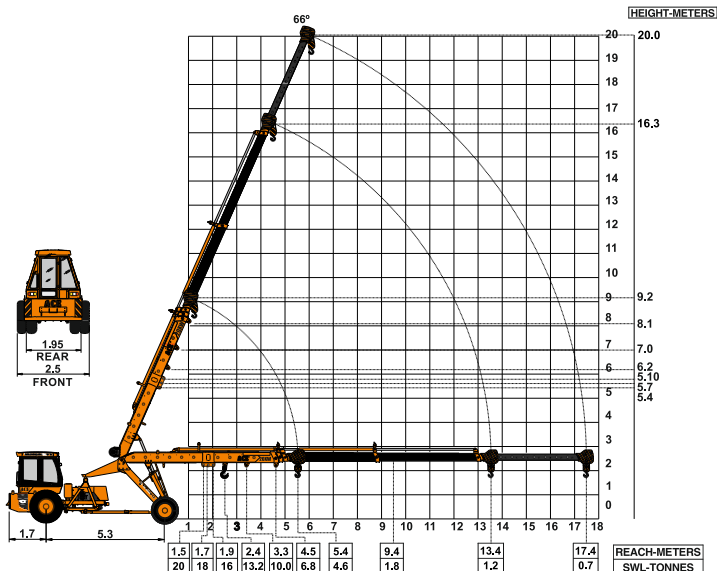
ACE 20XW 4-Part Boom (20 mtrs. height) Max. Capacity Manual Extension : 2 Tonnes
