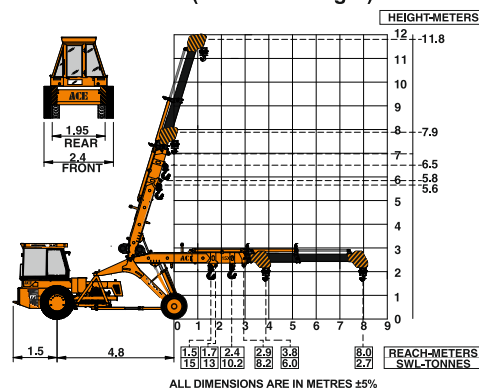
ACE 15XW Model Crane fitted with 3 Part boom (11.8 mtrs. height)
