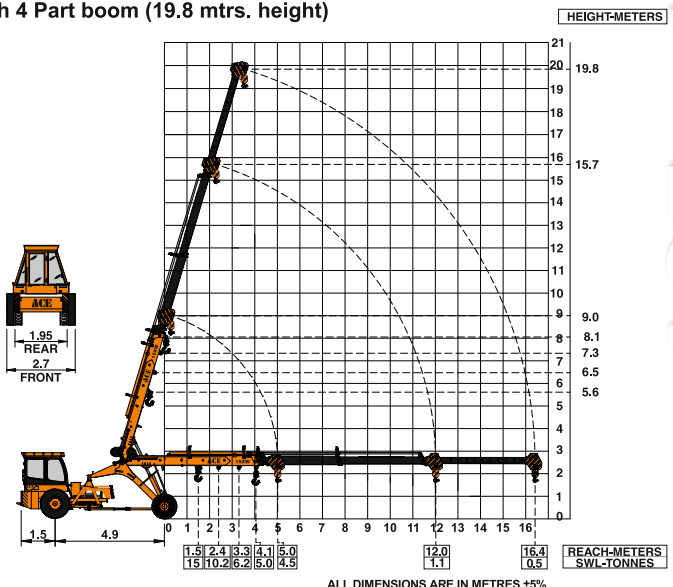
ACE 15XW Model Crane fitted with 4 Part boom (19.8 mtrs. height)
