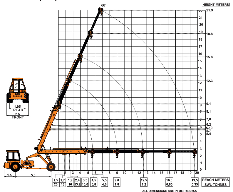
ACE 20XW 5-Part Boom (22 Mtrs. Height) Max. Capacity Manual Extension : 2 Tonnes
