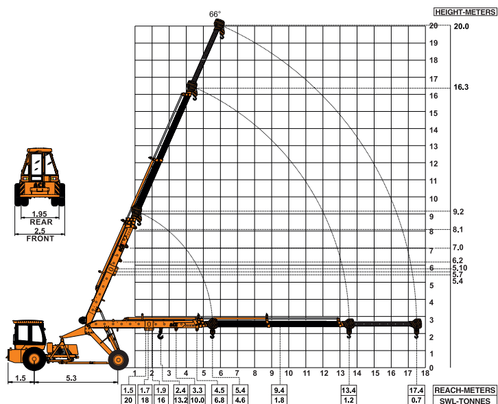
ACE 20XW 4-Part Boom (20 Mtrs. Height) Max. Capacity Manual Extension : 2 Tonnes
